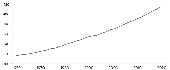
Concentrations of carbon dioxide, 1959–2020 (parts per million)
