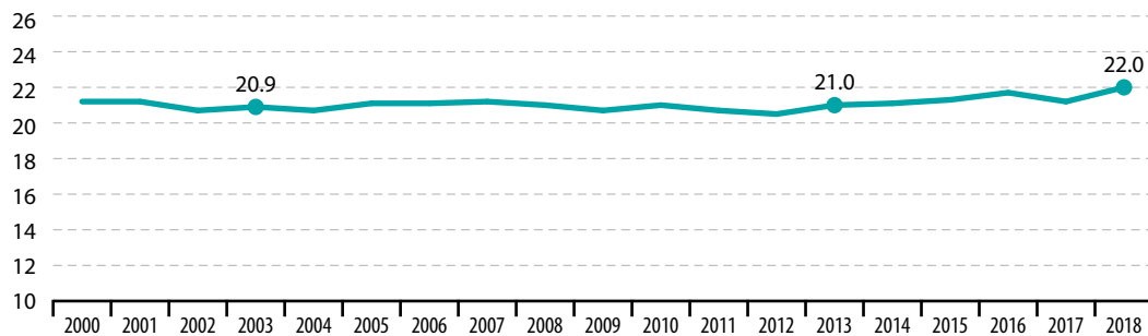
Figure 6.6: Nitrate in groundwater, EU, 2000–2018 ( \text{mg NO}_3 per litre)
