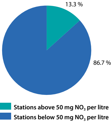
Figure 6.8: Share of groundwater measuring stations with nitrate concentrations above 50 mg/L, EU, 2012–2015 average (%)
