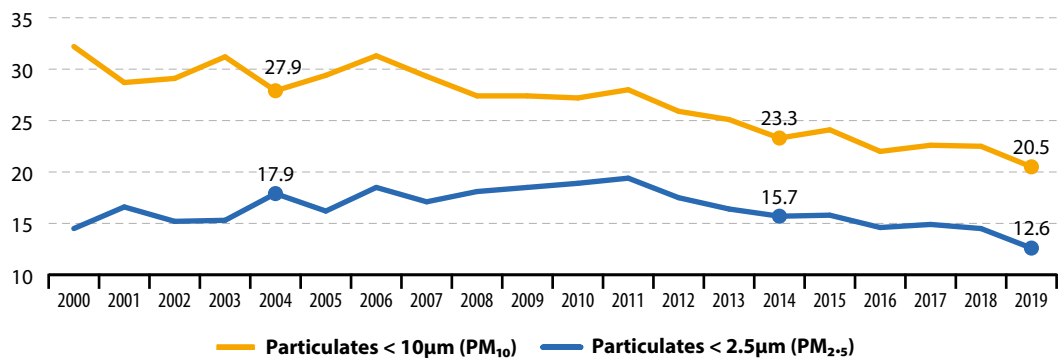
Figure 11.5: Exposure to air pollution by particulate matter, EU, 2000–2019 (µg/m 3 )
