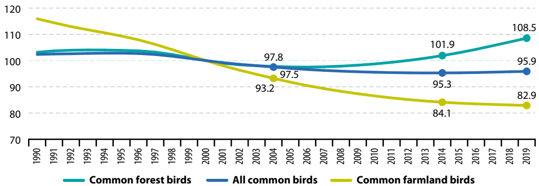
Figure 15.8: Common bird index, by type of species, EU, 1990–2019 (index 2000 = 100)
